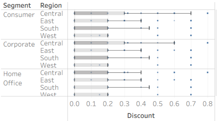
Box Plot
